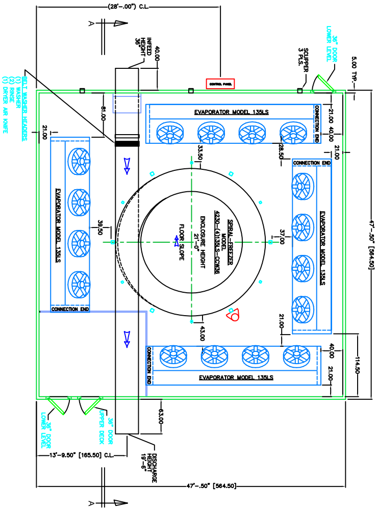
PLAN VIEW
